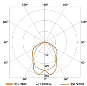
Light distribution curves for RS PRO DL 100
